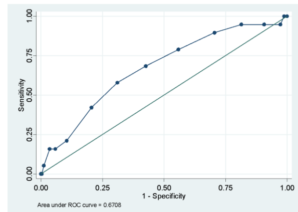
Figure 2. Area under the C curve of the Nutritional Risk F actor
