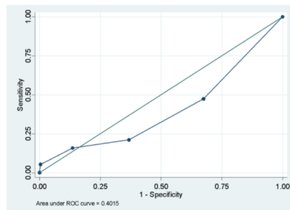
Figure 3. Area under the Curve of the Health Risk Factor
