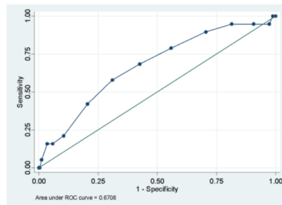
Figure 2. Area under the C curve of the Nutritional Risk F factor
